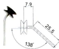
Lycra guide pulley without bearing wire \phi 2
