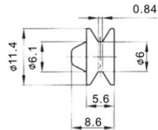
Lycra guide pulley without bearing wire \phi 2
