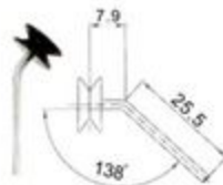
Lycra guide pulley without bearing wire \phi 2
