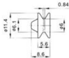
Lycra guide pulley without bearing wire \phi 2
