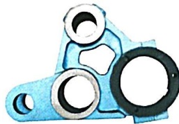
14 三孔轴架 Treble-hole bracket for O.E
