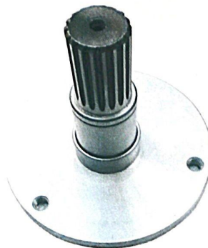
14 轴 Bobbin shaft for G.E
