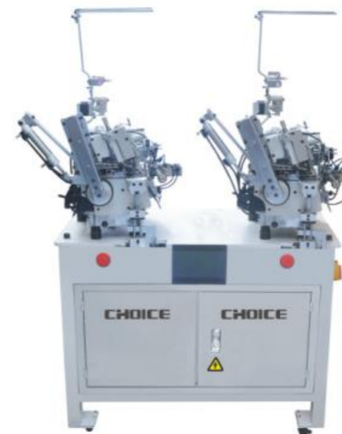
GC-5114EX-GLV AUTOMATIC GLOVE OVERLOCK MACHINE WITH ELASTIC INSERT
