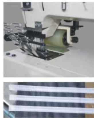
GC-1406PL 6-needle flat-bed double chain stitch sewing machine
