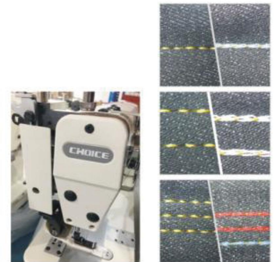
GC3802/2PL Chain stitch sewing machine with upper & down puller
