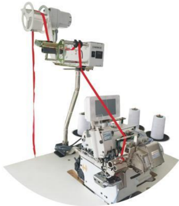
tape cutter with anti-stuck feeding device
