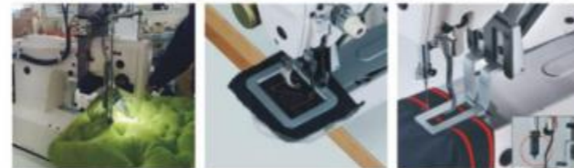
GC1908D holing bar tacking on cushion GC1905D program bar tacking Max. size: 50x60mm GC1904D pneumatic auto elastic joining bar tacking
